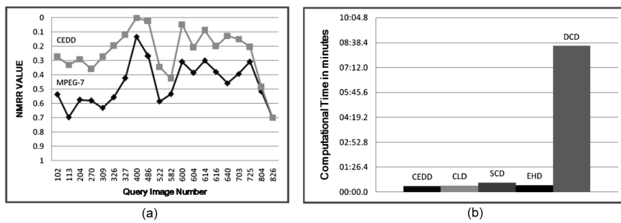
Fig. 5. (a) CEDD and MPEG-7 Average NMRR Values in Wang’s Database, (b) Descriptor Extraction Computational Time in Wang’s Image Database
